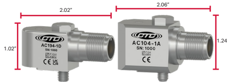
2 Pin Side Exit Compact vs. 2 Pin Side Exit Standard
